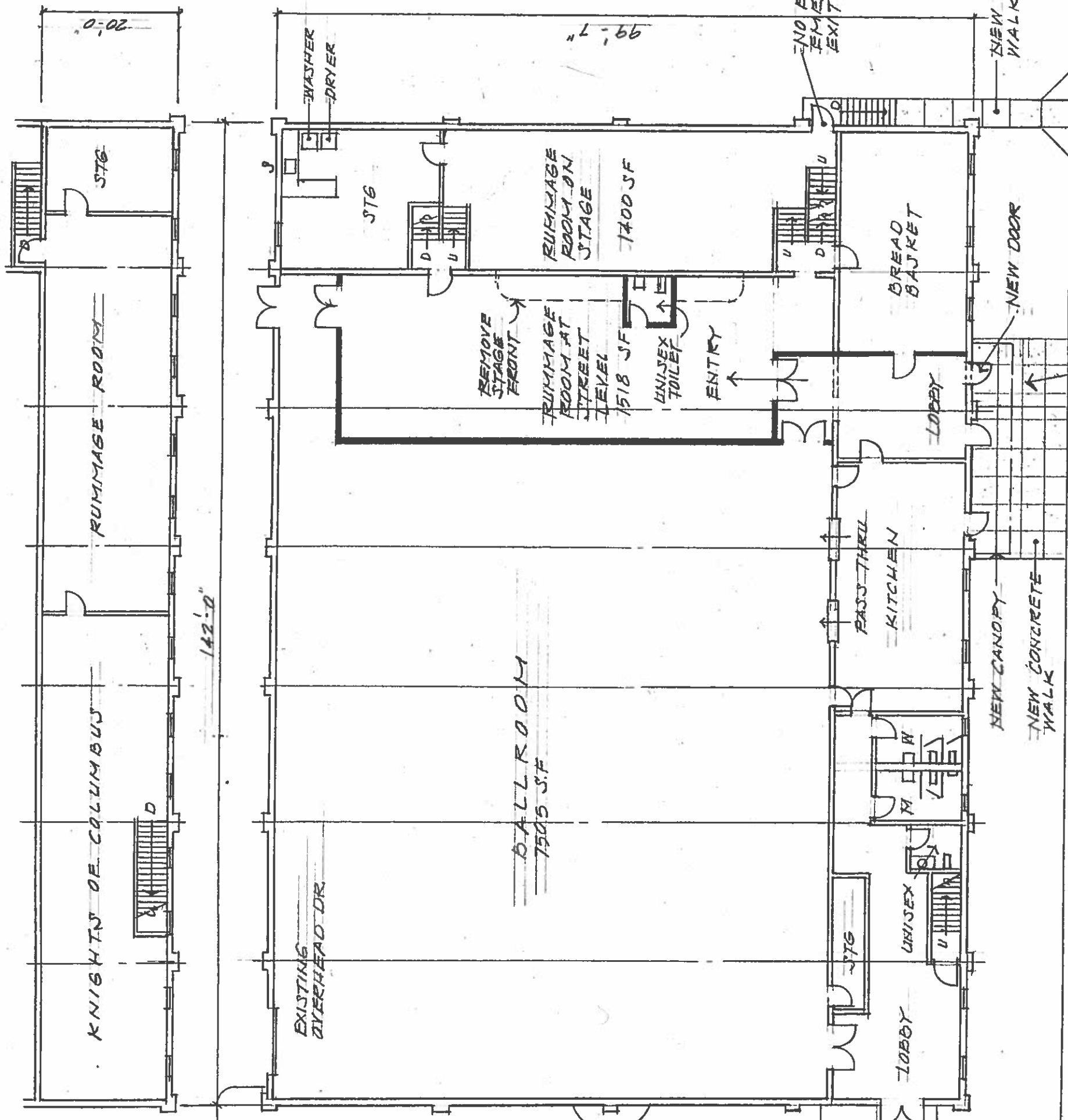
SECOND FLOOR PLAN 1/8" = 1'-0"
